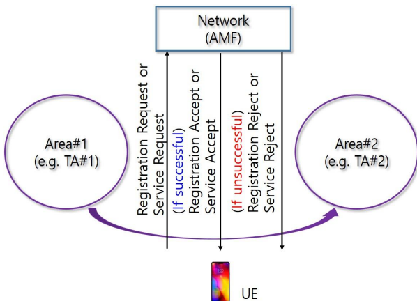
Fig. 2. Mobility Management in 5GS
