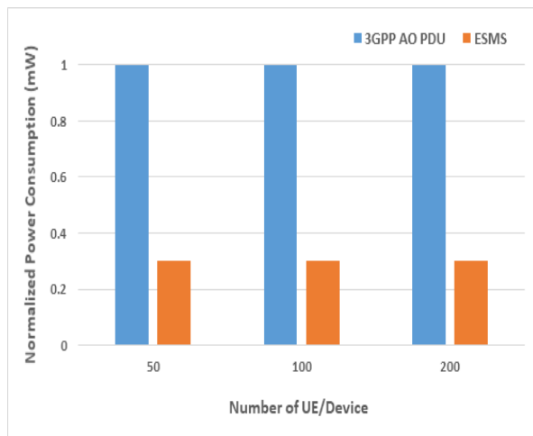
Fig. 5. Power consumption
