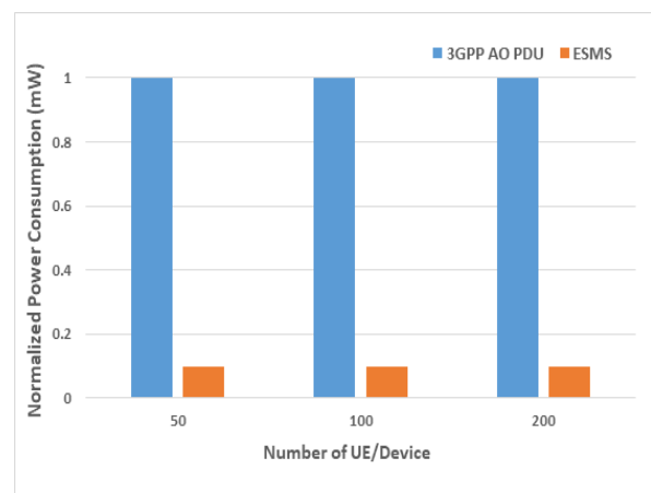
Fig. 6. Power consumption with backoff timer
