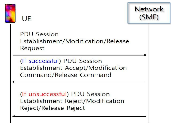
Fig. 3. Session Management in 5GS
