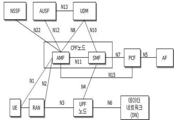
Fig. 1. 5G System(5GS) Architecture
