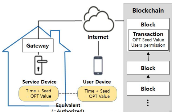
Fig. 5. System Architecture
