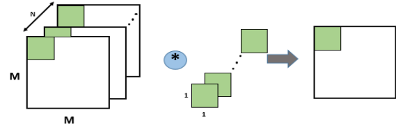
Fig. 2. Point-wise Convolution
