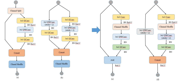
Fig. 5. Building blocks of our ShuffleDefectNet (c)(d). Old ShuffleNet V2 blocks (a)(b)
