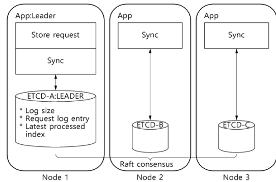
Fig. 1. Replication of Blockchain application
