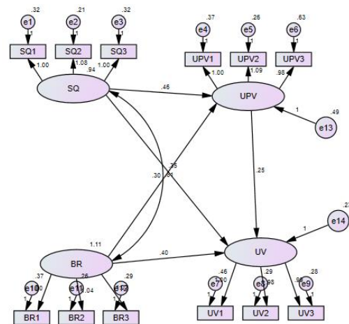
Fig. 2. Structural equation model
