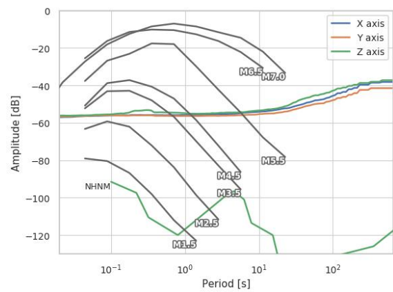
Fig. 4. Sensor noise floor @ lab environment
