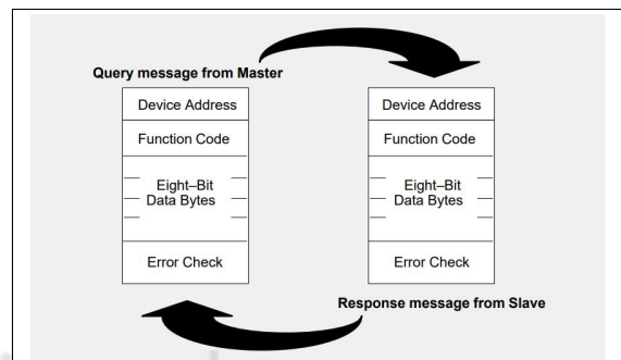
Fig. 3. Master-Slave Query-Response Cycle
