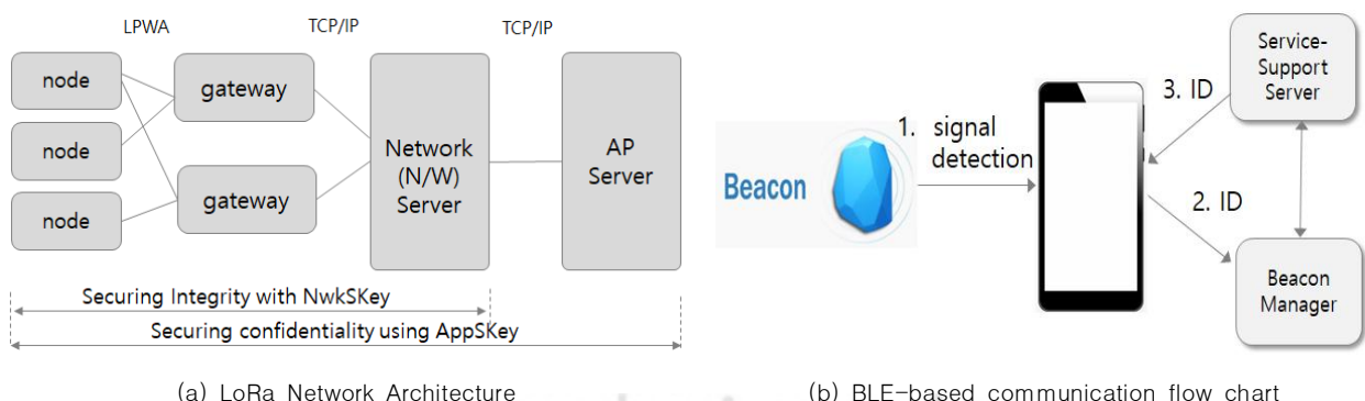
Fig. 1. Protocol for Support of Outdoor IoT Service
