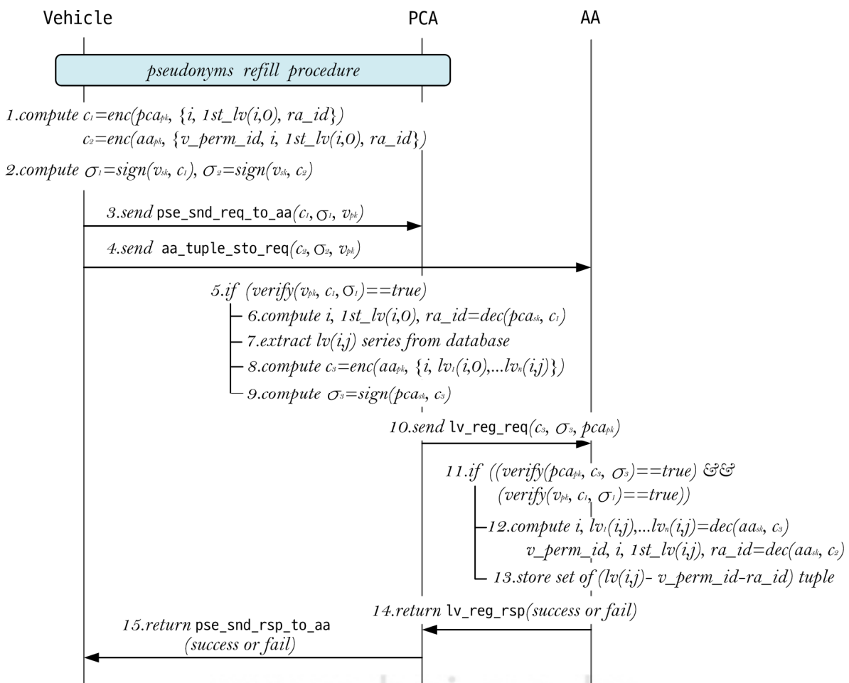
Fig. 1. Pseudonym Registration Protocol
