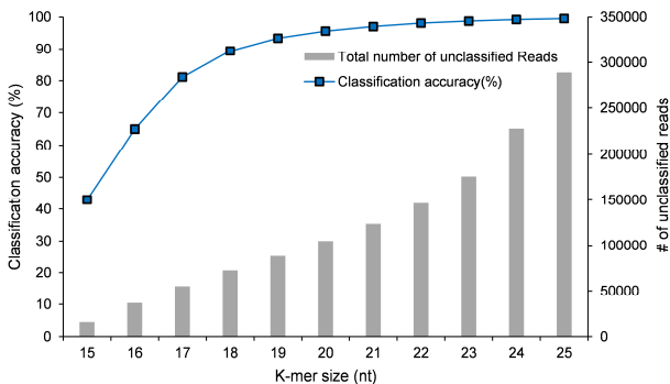
Fig. 5. Classification Performance
