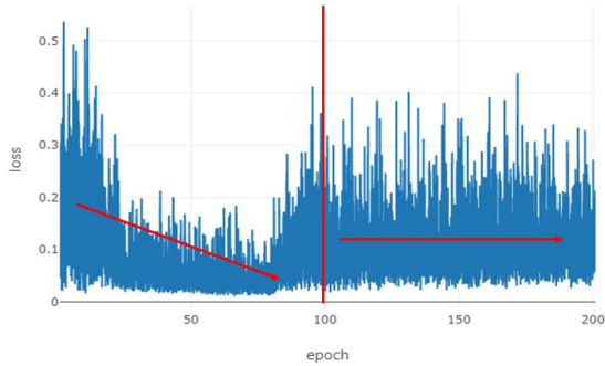
Fig. 3. Discriminator D_y 's loss according to epoch
