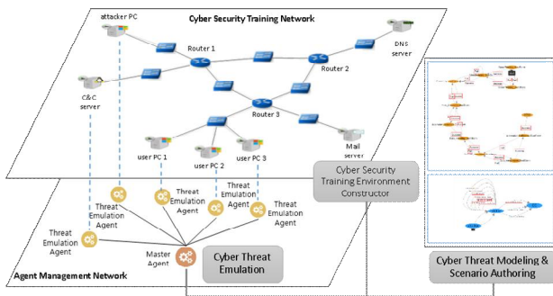
Fig. 1. CyTEA Overview
