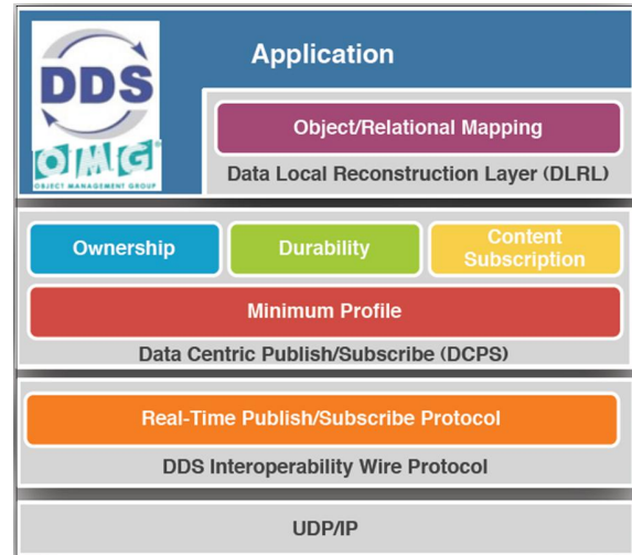
Fig. 1. DDS Architecture
