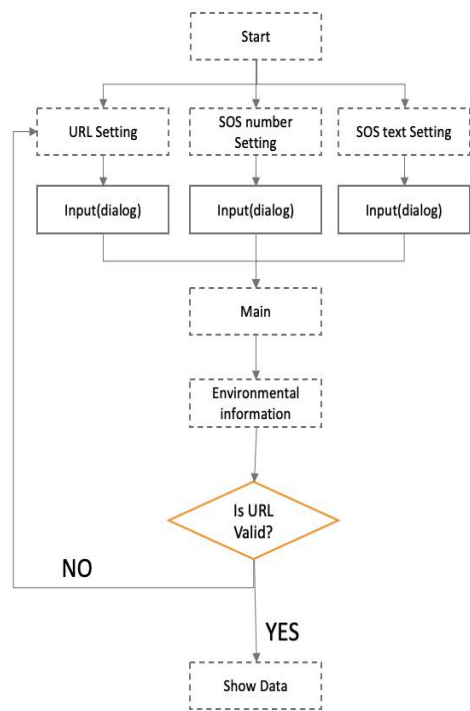
Fig. 3. Flowchart for Environmental Data
