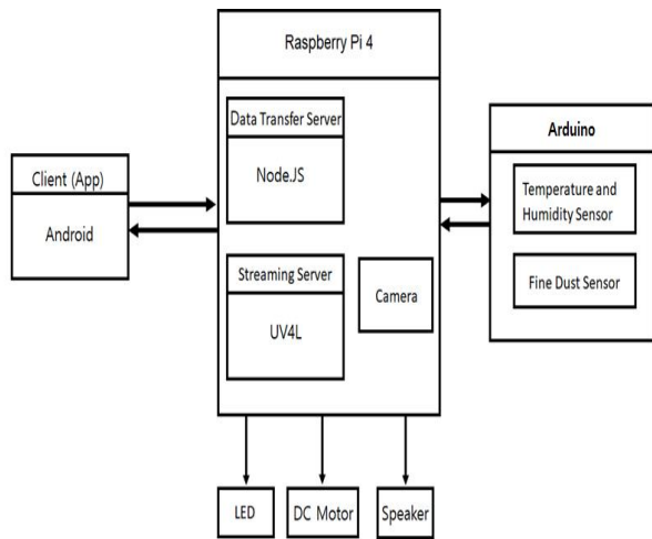
Fig. 1. System Configuration Diagram
