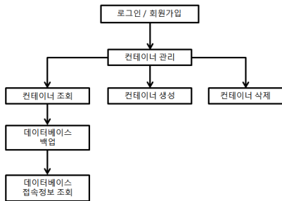
Fig. 3. Web system configuration (User)
