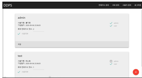
Fig. 9. User screen
