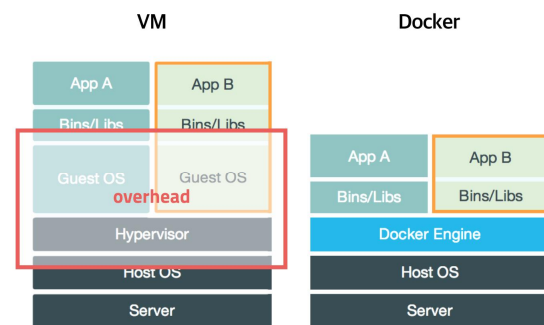
Fig. 2. Virtualization method of VM and Docker
