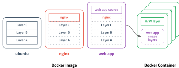
Fig. 1. Image layer storage method
