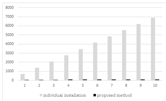
Fig. 13. Compare of individual installation and proposed method of Oracle 11g
