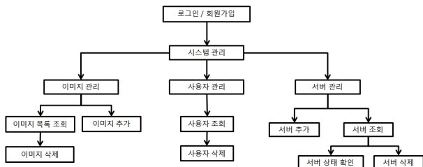
Fig. 4. Web system configuration (Administrator)
