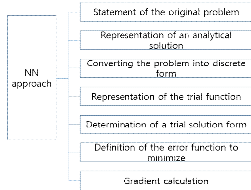
Fig. 3. Proposed neural network approach for singularity perturbed problem
