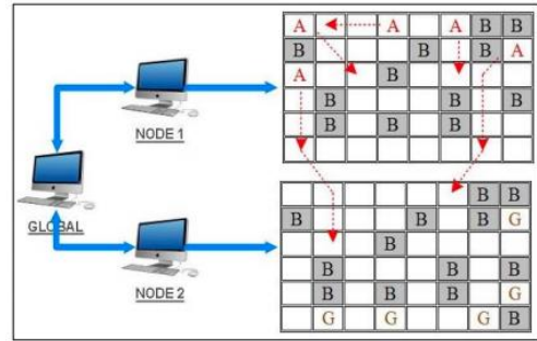
Fig. 4. Exploratory Trials by Multi-agent
