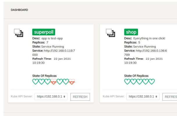
Fig. 9. BR2K Watch view after logging in
