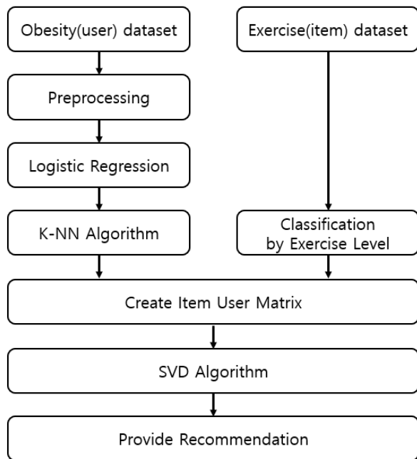
Fig. 3. Recommendation System Architecture
