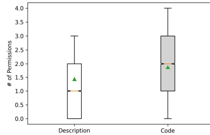
Fig. 4. Permission usages in app descriptions and code
