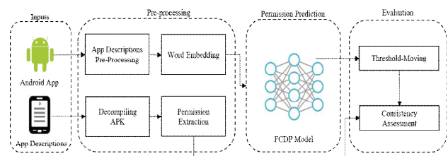
Fig. 1. Procedure of Methodology
