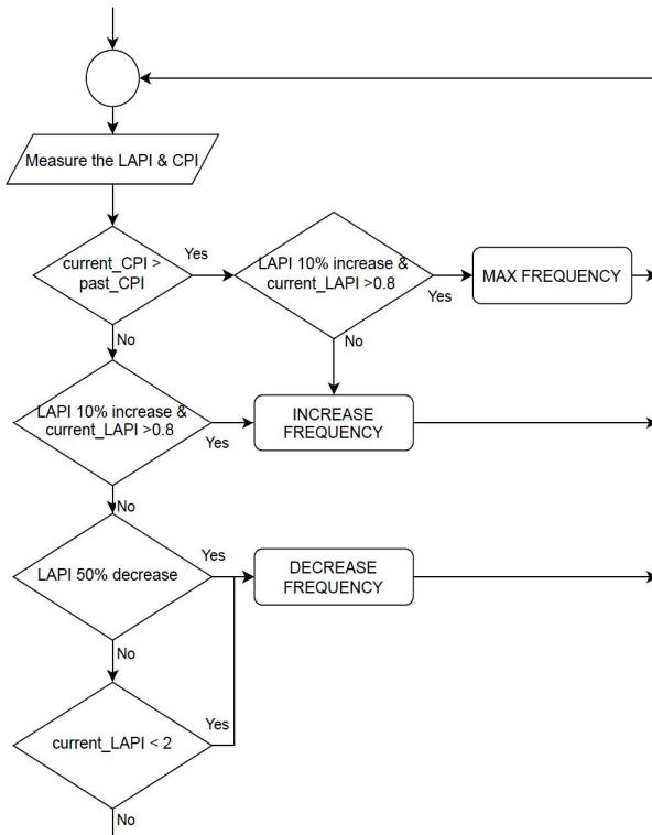
Fig. 8. eUFS flowchart
