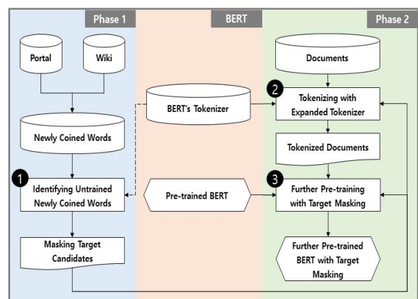
Fig. 2. Overview of the Proposed Methodology
