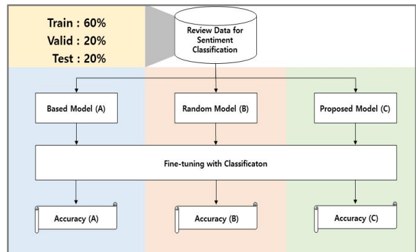
Fig. 9. Architecture of Sentiment Classification
