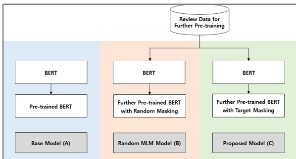
Fig. 8. Three Models for Performance Comparison
