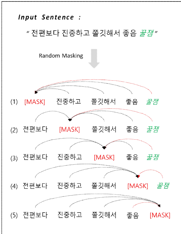
Fig. 1. MASK Candidates of Traditional MLM
