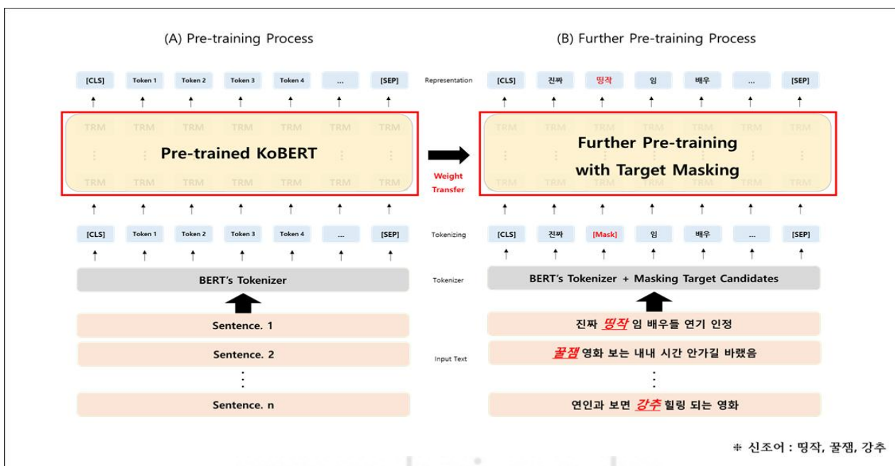
Fig. 7. Further Pre-training with Target Masking Model Process
