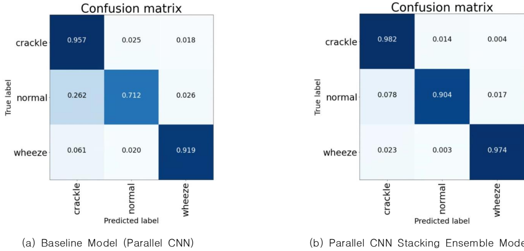
Fig. 10. Confusion matrix for the ensemble respiratory sound classification models : (a) (Baseline) Parallel CNN model analysis with Softmax Classifier; (b) Parallel CNN with Stacking Ensemble analysis
