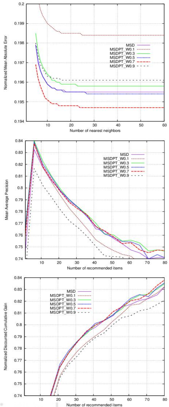
Fig. 1. Performance results using MovieLens
