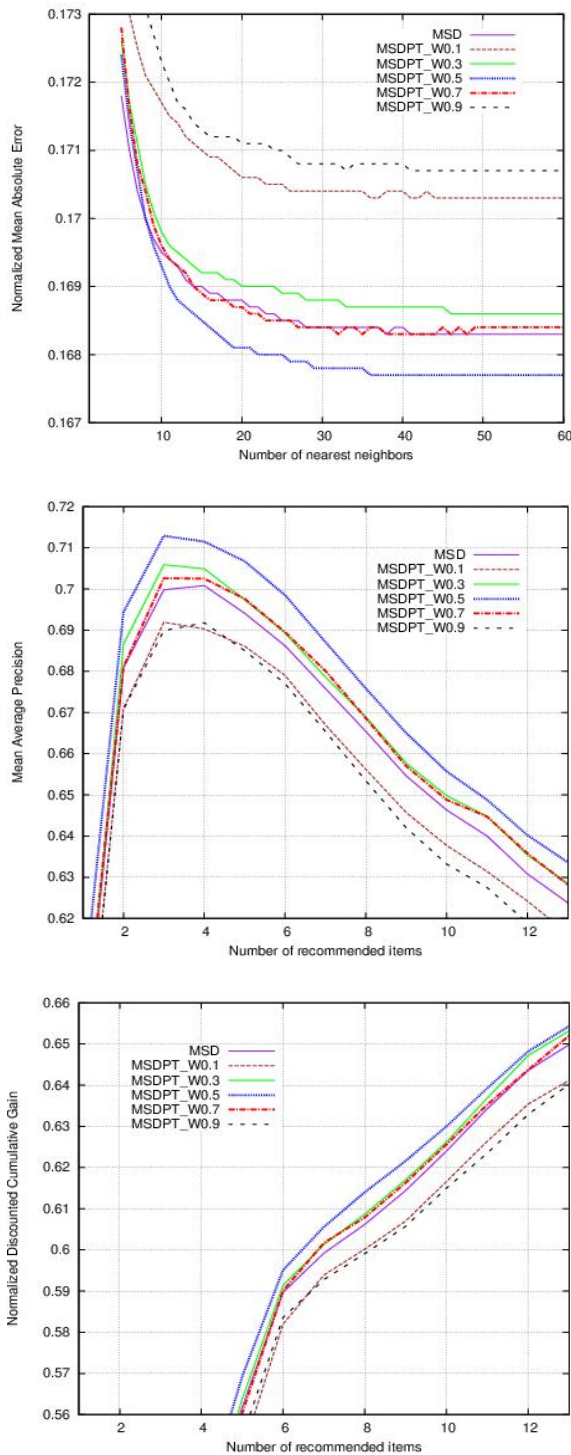
Fig. 2. Performance results using Jester
