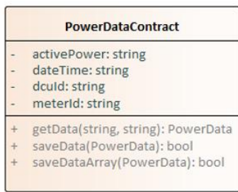
Fig. 3. Smart Contract Structure
