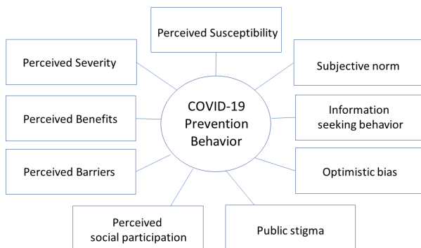
Fig. 1. Research Model
