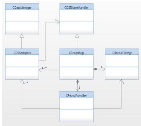
Fig. 11. User Pattern Record Class Diagram
