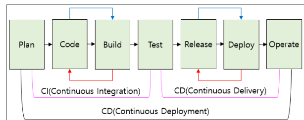
Fig. 1. DevOps Phases
