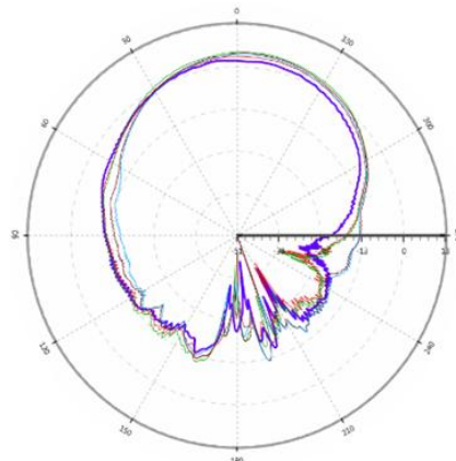
Fig. 13. Measured 2-D co-pol. radiation patterns when feeding point is port 2 at the 1×2 array antenna(Pol.-V)
