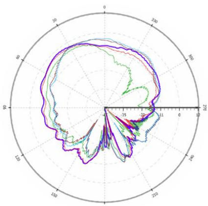
Fig. 12. Measured 2-D cross-pol. radiation patterns when feeding point is port 1 at the 1×2 array antenna(Pol.-H)
