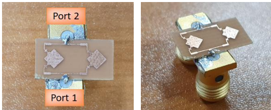
Fig. 7. Prototype of the proposed 1x2 array antenna
