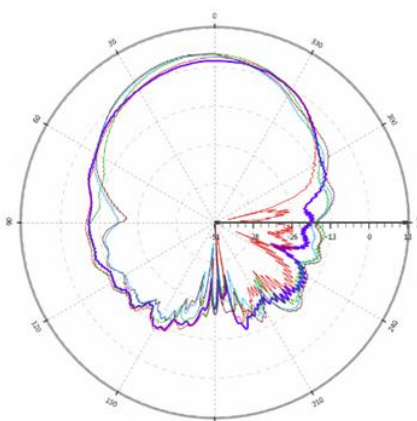
Fig. 15. Measured 2-D co-pol. radiation patterns when feeding point is port 2 at the 1×2 array antenna(Pol.-H)
