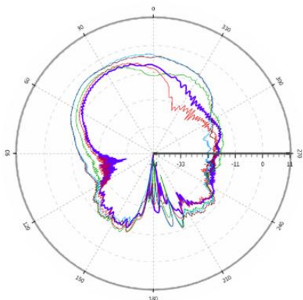
Fig. 10. Measured 2-D radiation patterns when feeding point is port 1 at the 1×2 array antenna(Pol.-V)
