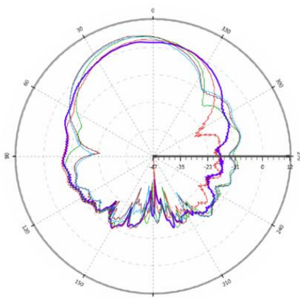
Fig. 11. Measured 2-D co-pol. radiation patterns when feeding point is port 1 at the 1×2 array antenna(Pol.-H)
