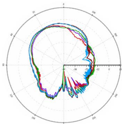
Fig. 14. Measured 2-D cross-pol. radiation patterns when feeding point is port 2 at the 1×2 array antenna(Pol.-V)
