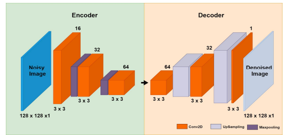
Fig. 2.1 CAE architecture for image denoising
