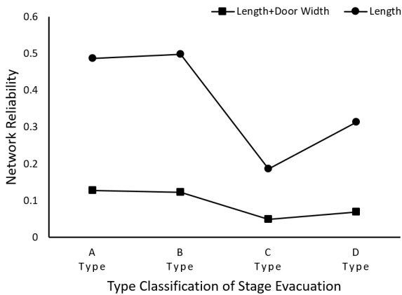
Fig. 7. Network Reliability by Stage Evacuation Type
