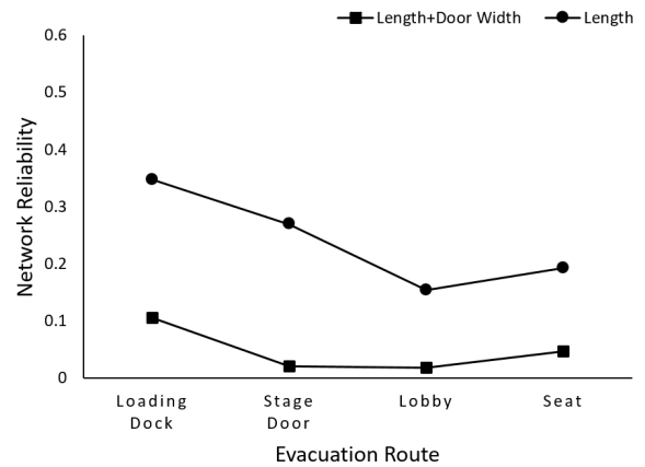
Fig. 6. Network Reliability by Evacuation Direction
