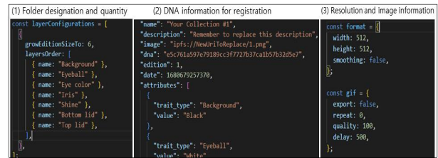
Fig. 10. Creation of NFT index content
