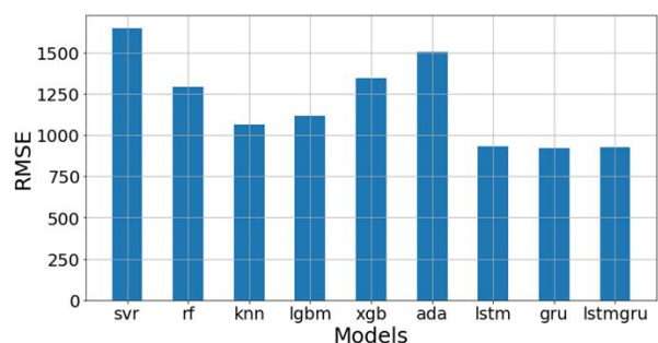
Fig. 4. Comparison of RMSE between algorithms using the close of 15 days or 1 day
