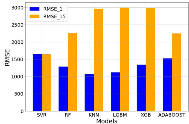
Fig. 3. RMSE of non-time-series models using the close of 15 days or 1 day
