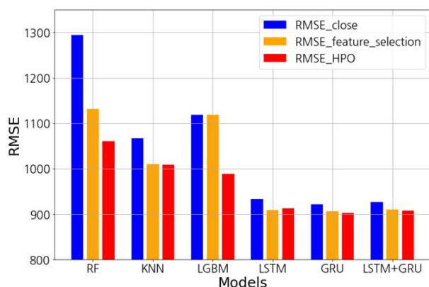
Fig. 6. RMSE of feature selection and hyperparameter tuning
