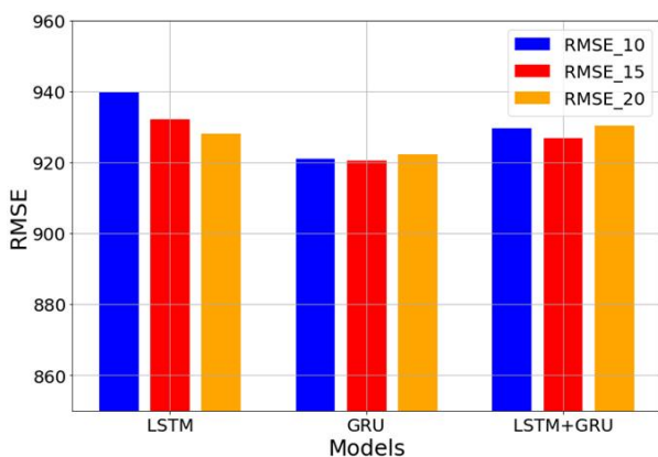
Fig. 2. RMSE Comparison of 10 days, 15 days, 20 days close of time-series models
