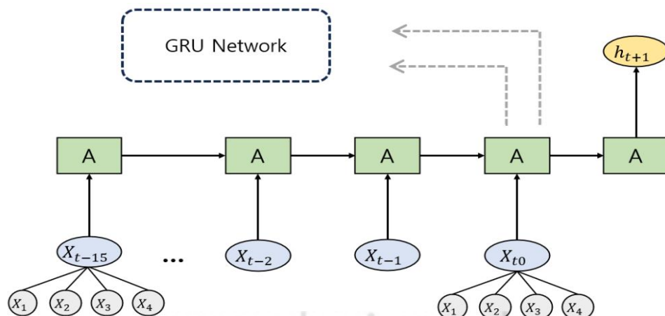
Fig. 5. GRU Network with optimal combination
