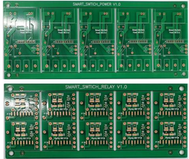
Fig. 6. Power Board(Top) and Relay Board(Bottom) Sample
