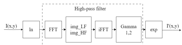
Fig. 1. Homomorphic filtering flowchart
