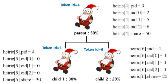
Fig. 8. Example of NFT hierarchy and the 'hieric' structure values
