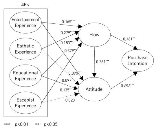
Fig. 1. Results of Path Analysis
