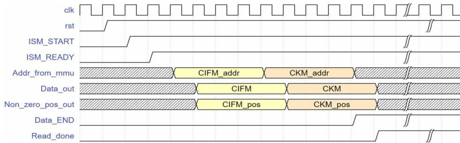
Fig. 5. Data Control Module Timing Diagram
