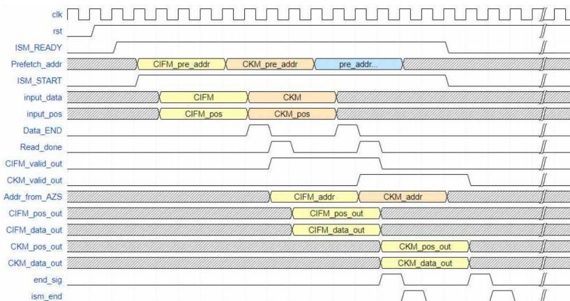
Fig. 7. Data Prefetch Module Timing Diagram
