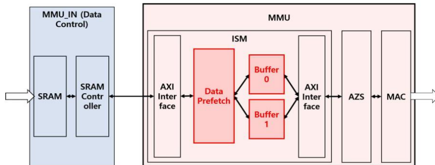
Fig. 4. System Architecture with Data Prefetch
