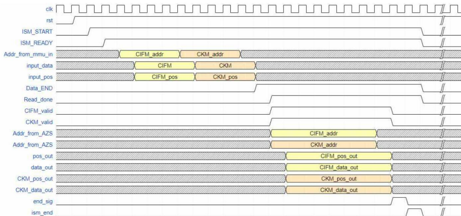
Fig. 6. ISM Module Timing Diagram
