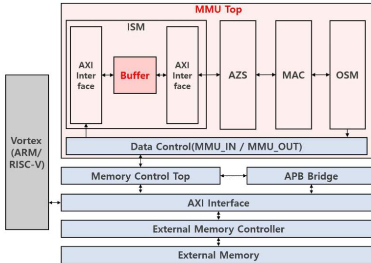
Fig. 2. System Architecture
