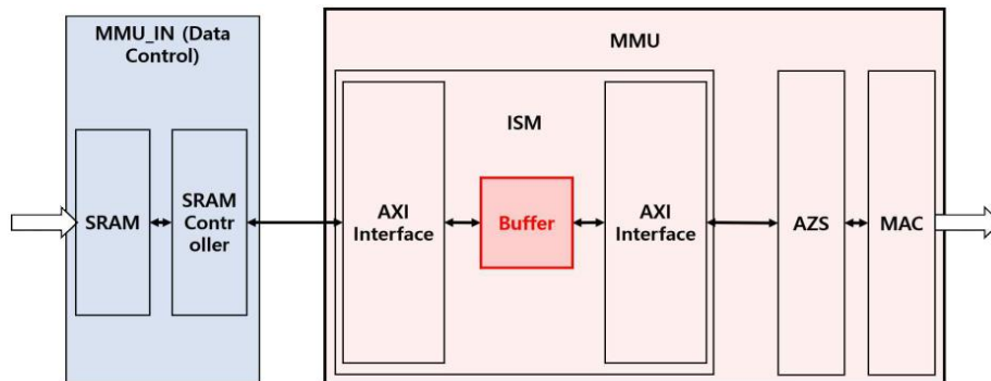
Fig. 3. System Architecture without Prefetch
