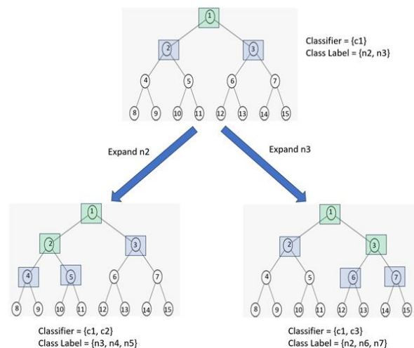
Fig. 2. Intuitive example of node expansion
