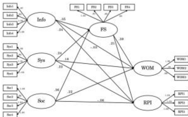
Fig. 2. Path diagram
