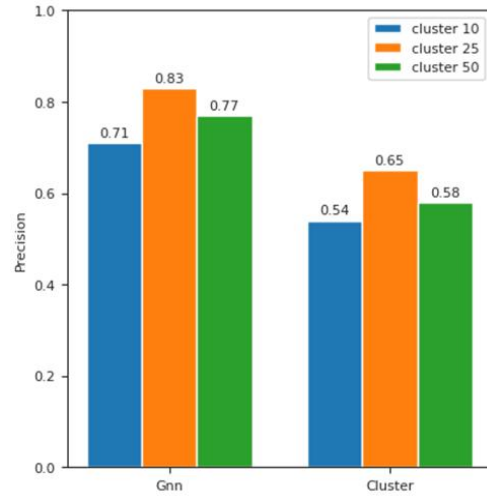
Fig. 5. Experiments on Precision in Real
