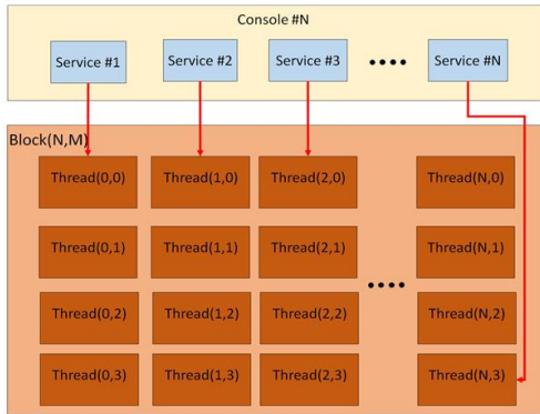
Fig. 12. Matching Method of Service #1
