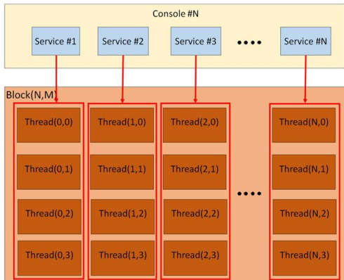
Fig. 13. Matching Method of Service #2
