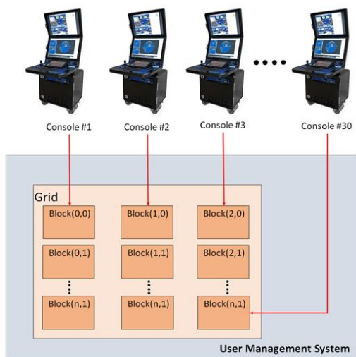
Fig. 11. Console and Block Allocation Method
