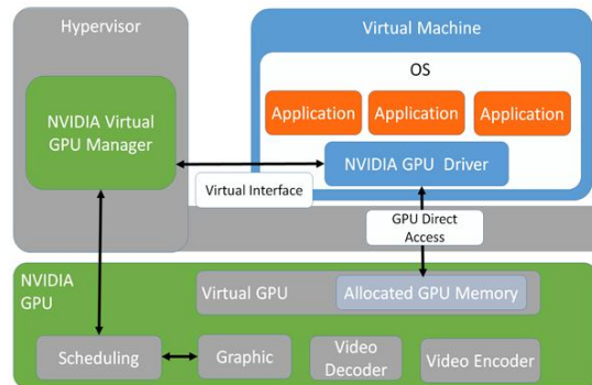
Fig. 7. Virtual GPU Architecture
