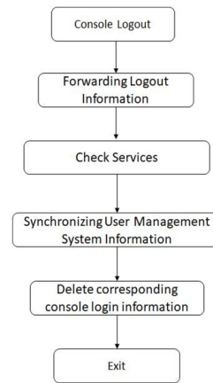
Fig. 9. Logout Flow Chart
