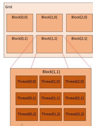
Fig. 10. GPU Architecture
