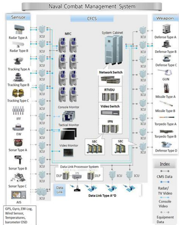
Fig. 1. Combat Fire Command System
