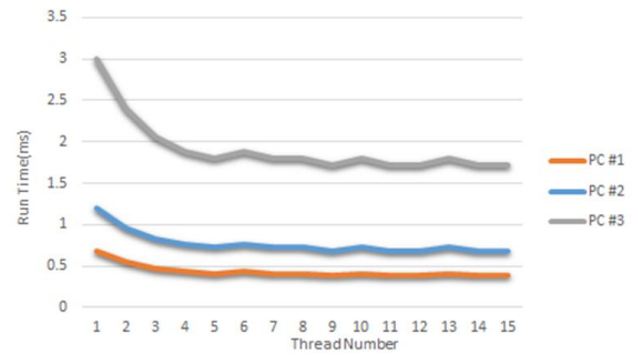
Fig. 14. Run Time according to Thread
