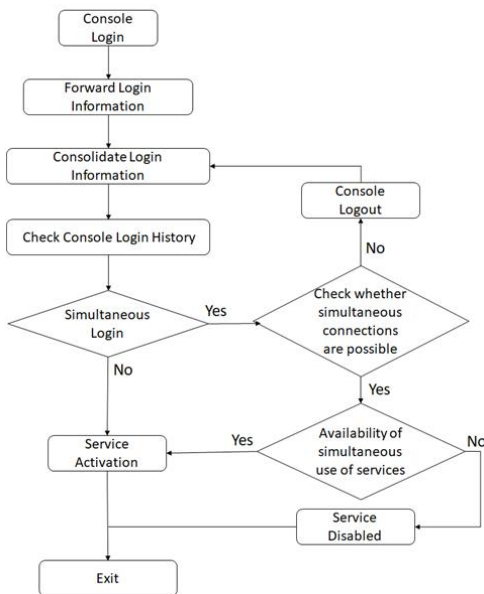
Fig. 8. User Management Method Flow Chart
