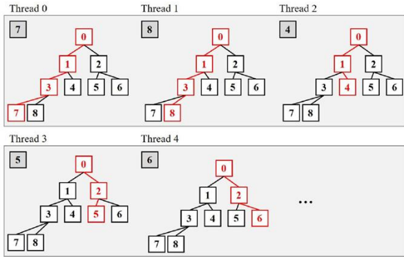
Fig. 7. Depth-first search on GPU.
