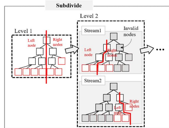
Fig. 2. Node subdivision.
