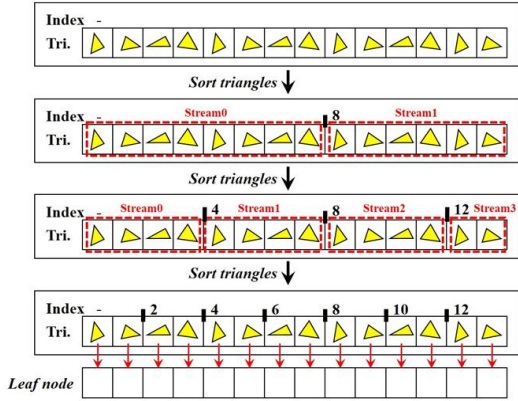
Fig. 3. BVH construction.
