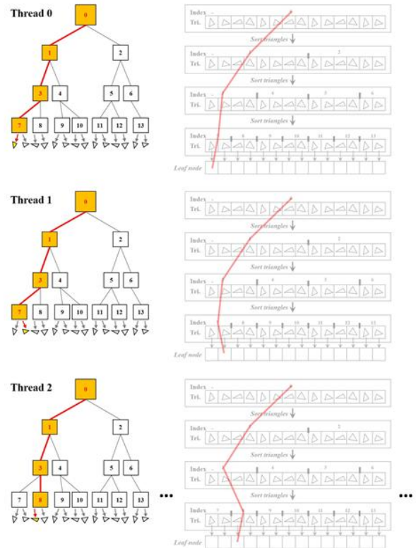
Fig. 6. Collision detection.
