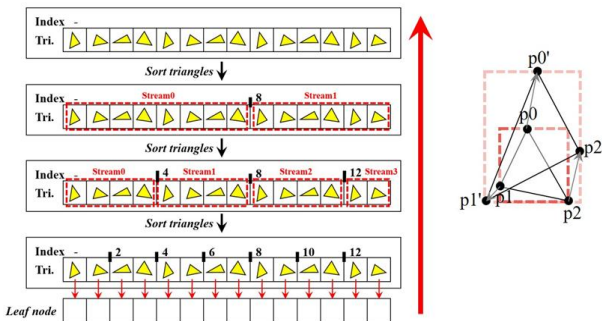
Fig. 4. Refitting BVH.
