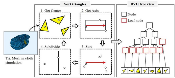
Fig. 1. An overview of GPU-based BVH tree construction.
