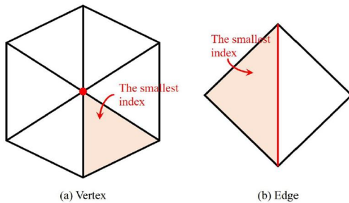
Fig. 8. Collision candidates collected based on the R-triangle.
