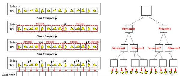
Fig. 5. Tree visualization of BVH.
