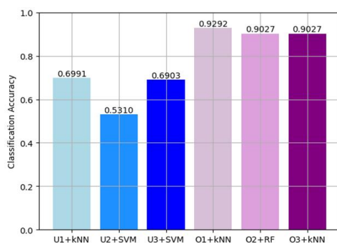
Fig. 8. The Highest Accuracies among All Combinations in Ablation Study 3
