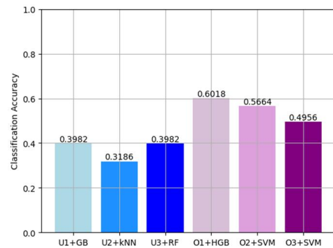
Fig. 7. The Highest Accuracies among All Combinations in Ablation Study 2
