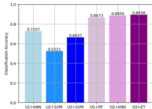
Fig. 6. The Highest Accuracies among All Combinations in Ablation Study 1
