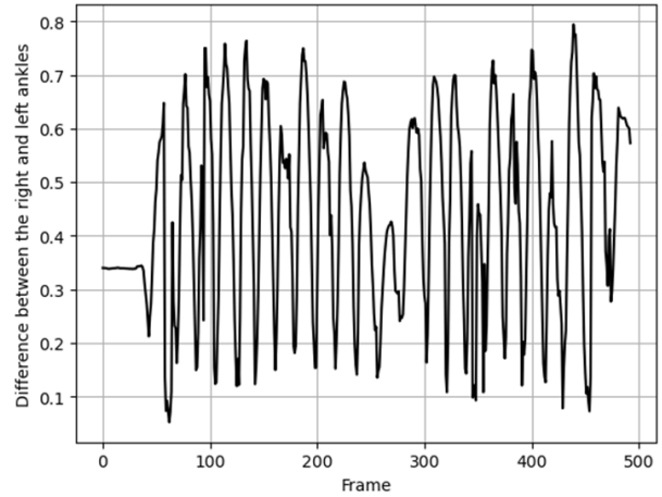
Fig. 4. Trajectory of \text{Diff}[n] During Walking
