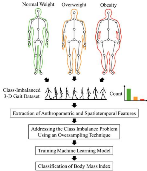
Fig. 1. Schematic Overview of the Proposed Method
