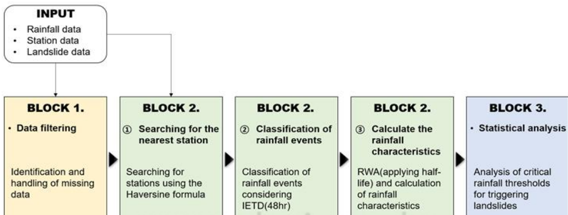
Fig. 2. Logical framework of the algorithm
