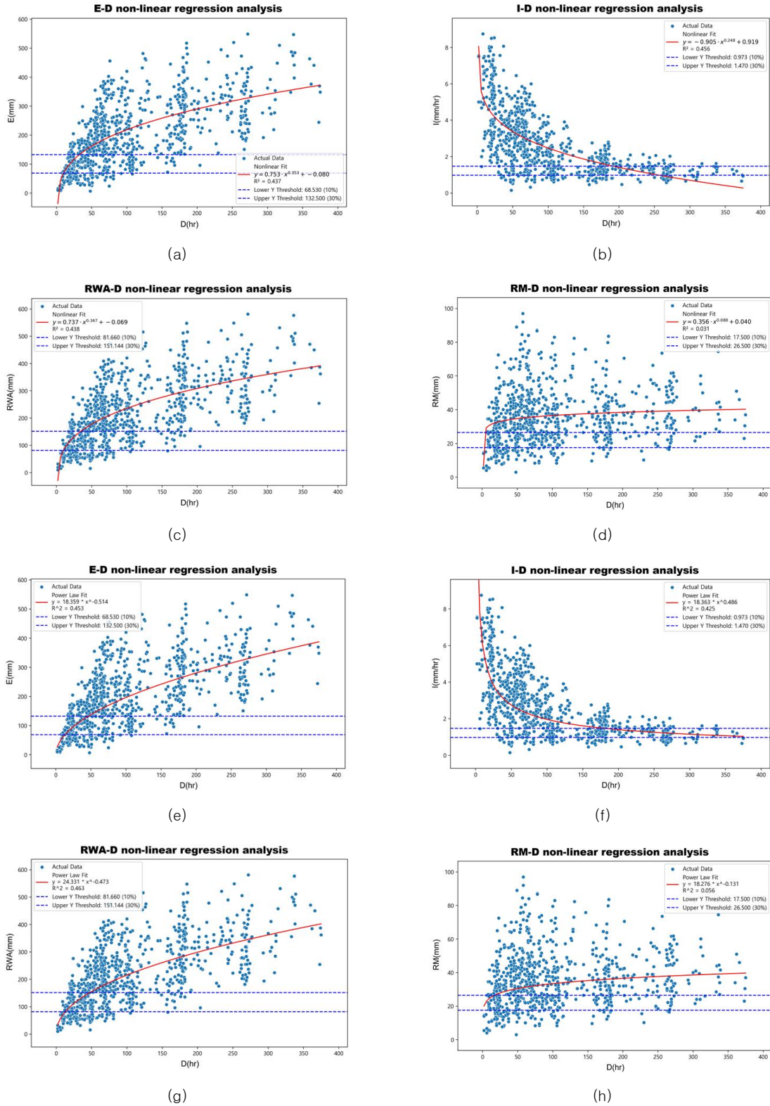
Fig. 5. Results of non-linear regression and power law regression analysis. (a): non-linear E-D curve, (b): non-linear I-D curve, (c): non-linear RWA-D, (d): non-linear RM-D, (e): power law E-D curve, (f): power law I-D curve, (g): power law RWA-D curve, (h): power law RM-D curve
