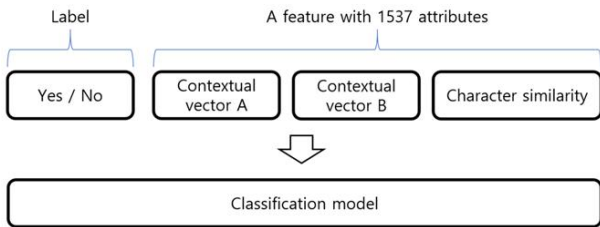
Fig. 3. Label and features used by classification models to determine the same formula given two mentions
