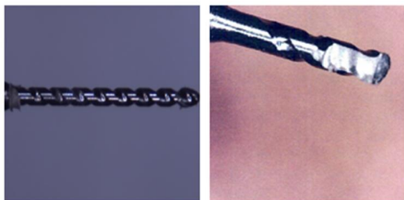
Fig. 8. Normal and defective drill bits
