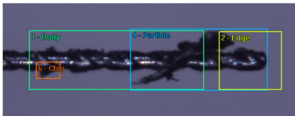
Fig. 9. Drill bit foreign matter inspection system
