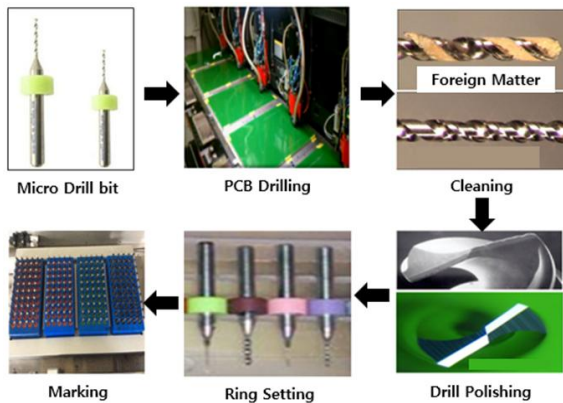
Fig. 2. Drill bit re-sharpening process
