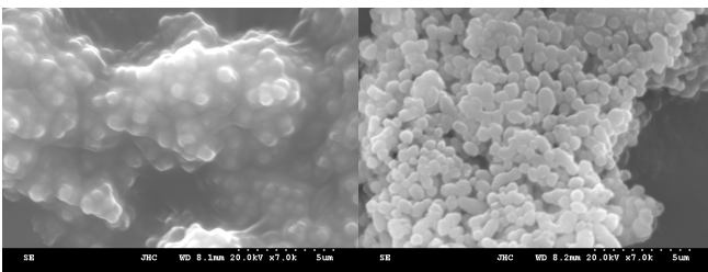
Fig.3. Scanning electron micrography of supra gingival biofilm.
