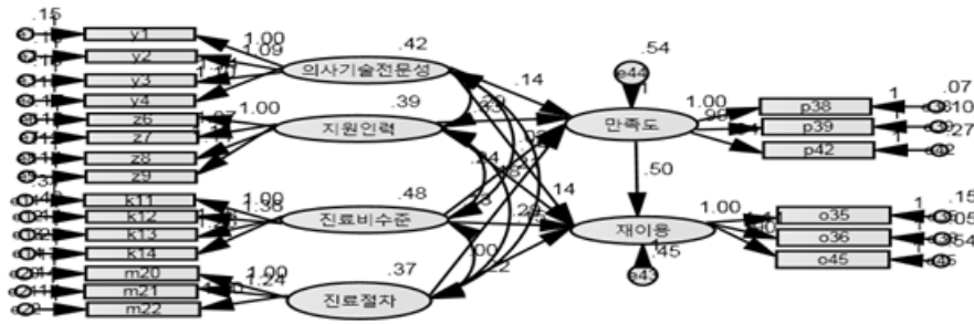
Fig. 1. Path diagram of covariance structural model
