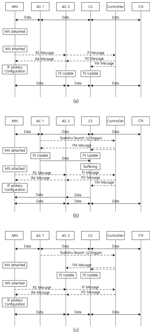
[Fig. 2] QoS-based handover procedure.
